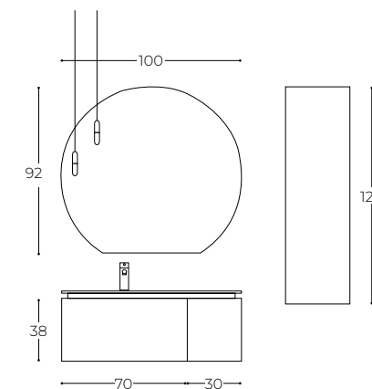
L 100 (70+30) H 38 P 46
