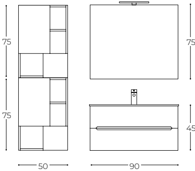
L 90 H 45 P 46
