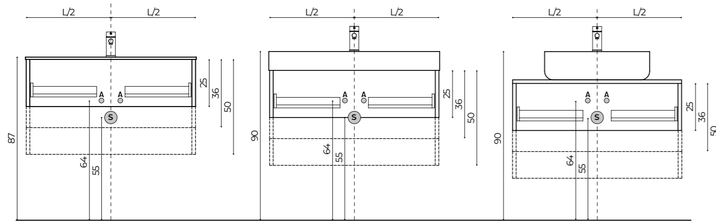
QUOTE BASI PORTALAVABO CX H.25, H.36, H.50 QUOTAS DISCHARGES BASE UNIT FOR WASHBASIN CX H.25, H.36, H.50
